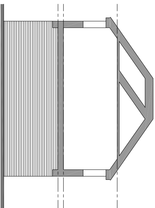
Existing Section / Elevation thru Alley/Ginnel
